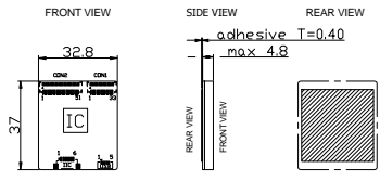
CONTROL BOARD
